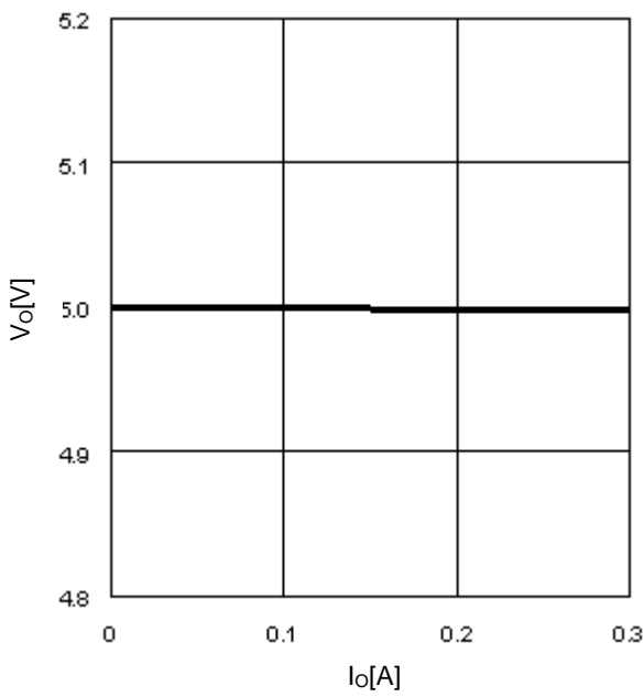
Figure 25. I_o - V_o
