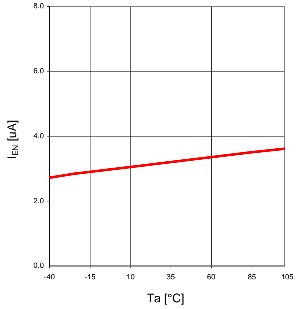
Figure 24. Ta- I_{EN}
